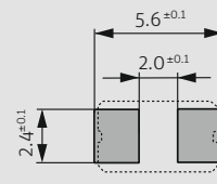
pad layout
