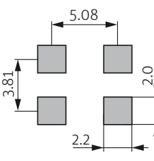
pad layout
