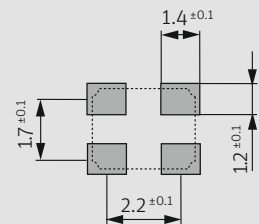
pad layout
